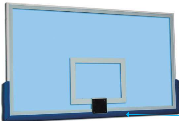
Art. S04206 / S04208 Coppia tabelloni in Plexiglass trasparente oppure in cristallo temperato dimensioni cm. 180x105 - compreso telaio e protezione Pair of basketball boards in trasparent acrylic or tempered glass 180x105 cm. mounted onto varnished steel frame with pads
